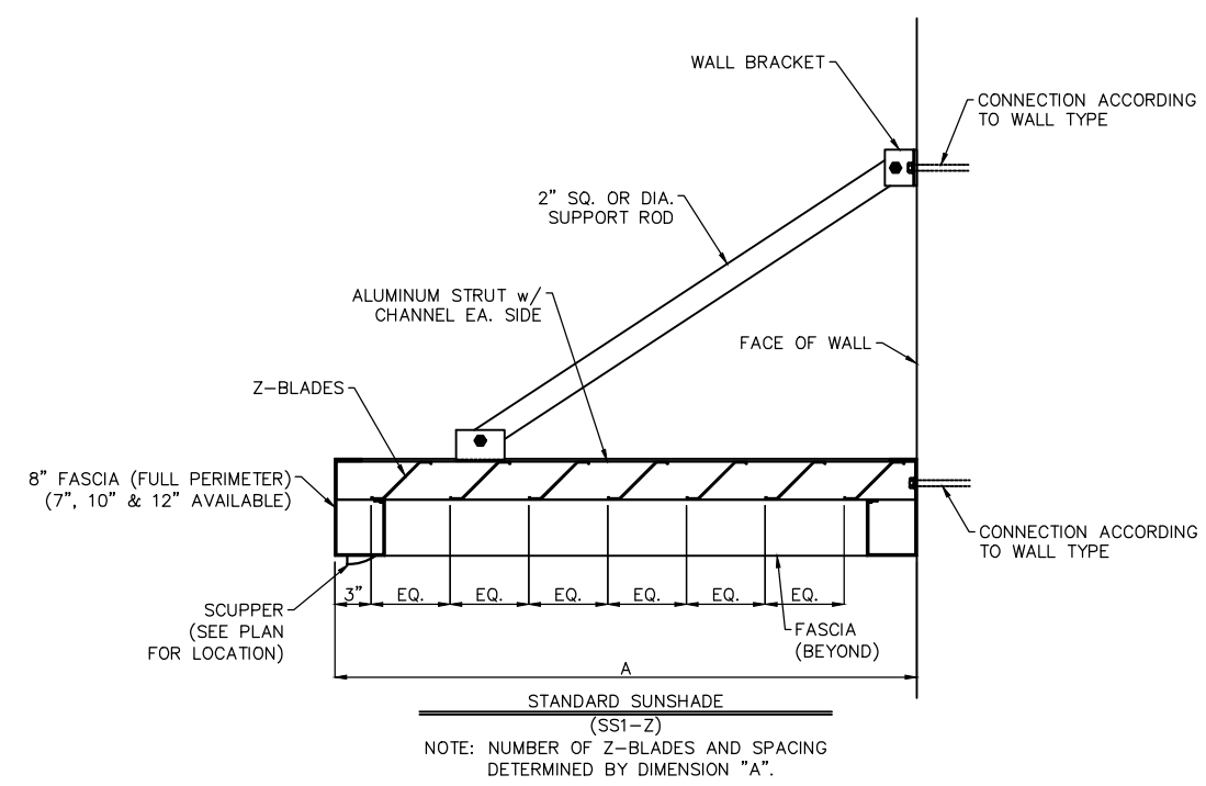
TYPICAL 2"x2" SUNSHADE DETAIL
