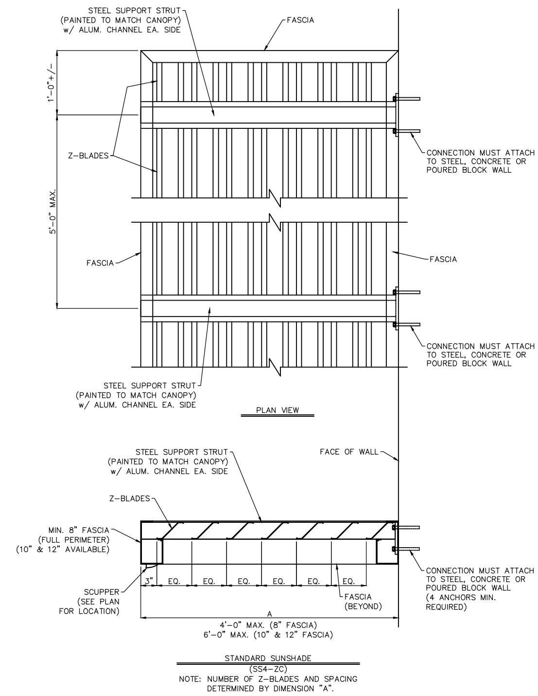
CANTILEVERED SUNSHADE DETAIL
