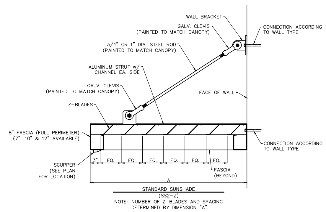
TYPICAL ROD & CLEVIS SUNSHADE DETAIL
