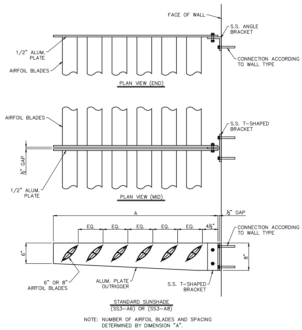
CANTILEVERED SUNSHADE DETAIL
